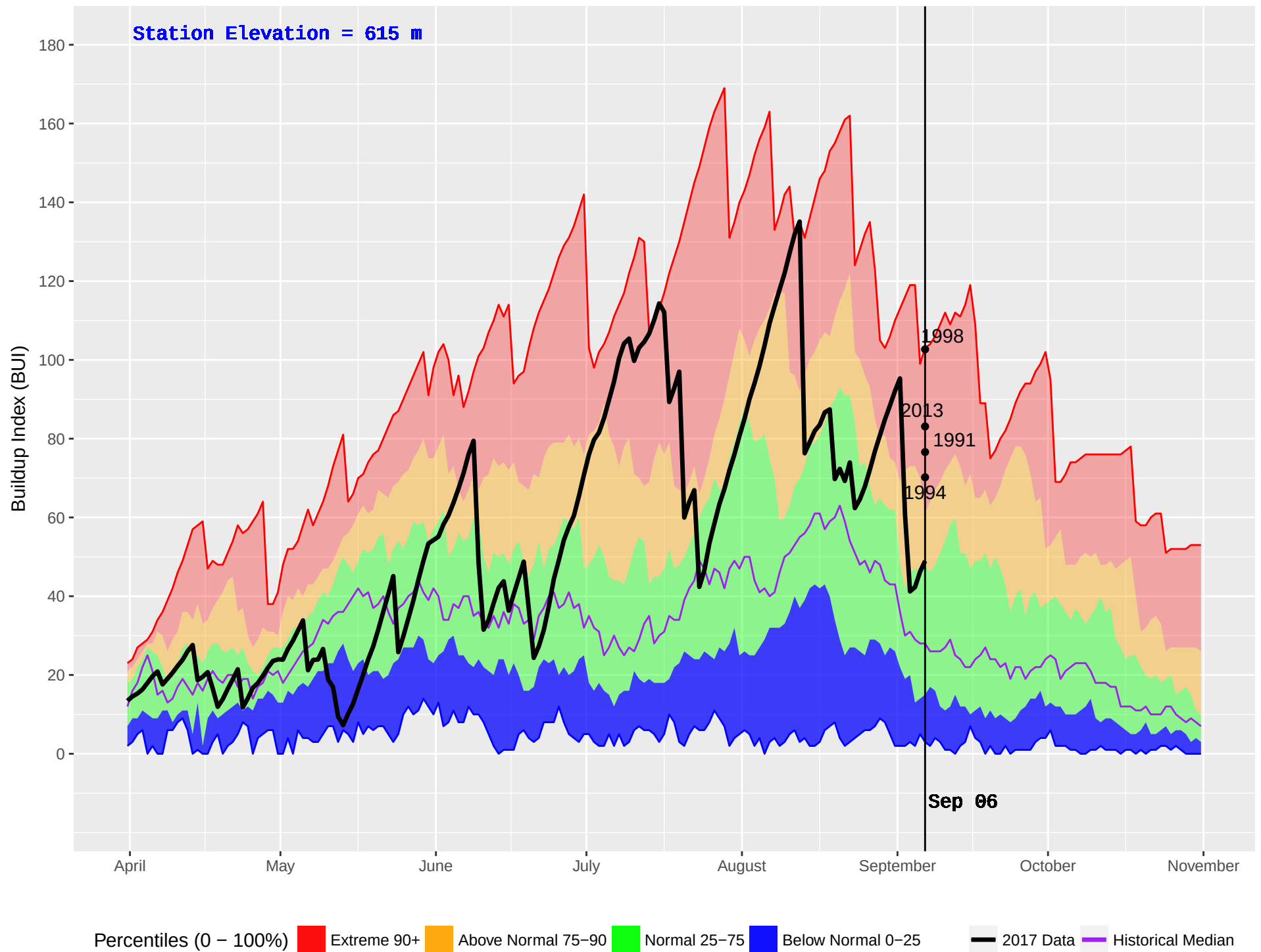
HIXON (187) : Historical (1976–2016) and Current (2017) Noon Buildup Index (BUI)
