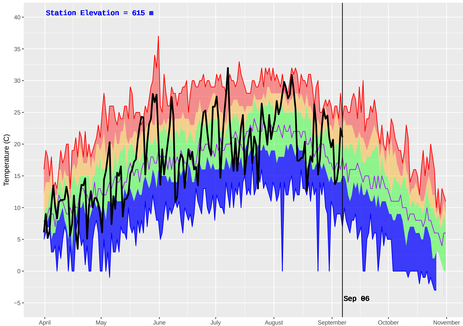
HIXON (187) : Historical (1976–2016) and Current (2017) Noon Temperature
