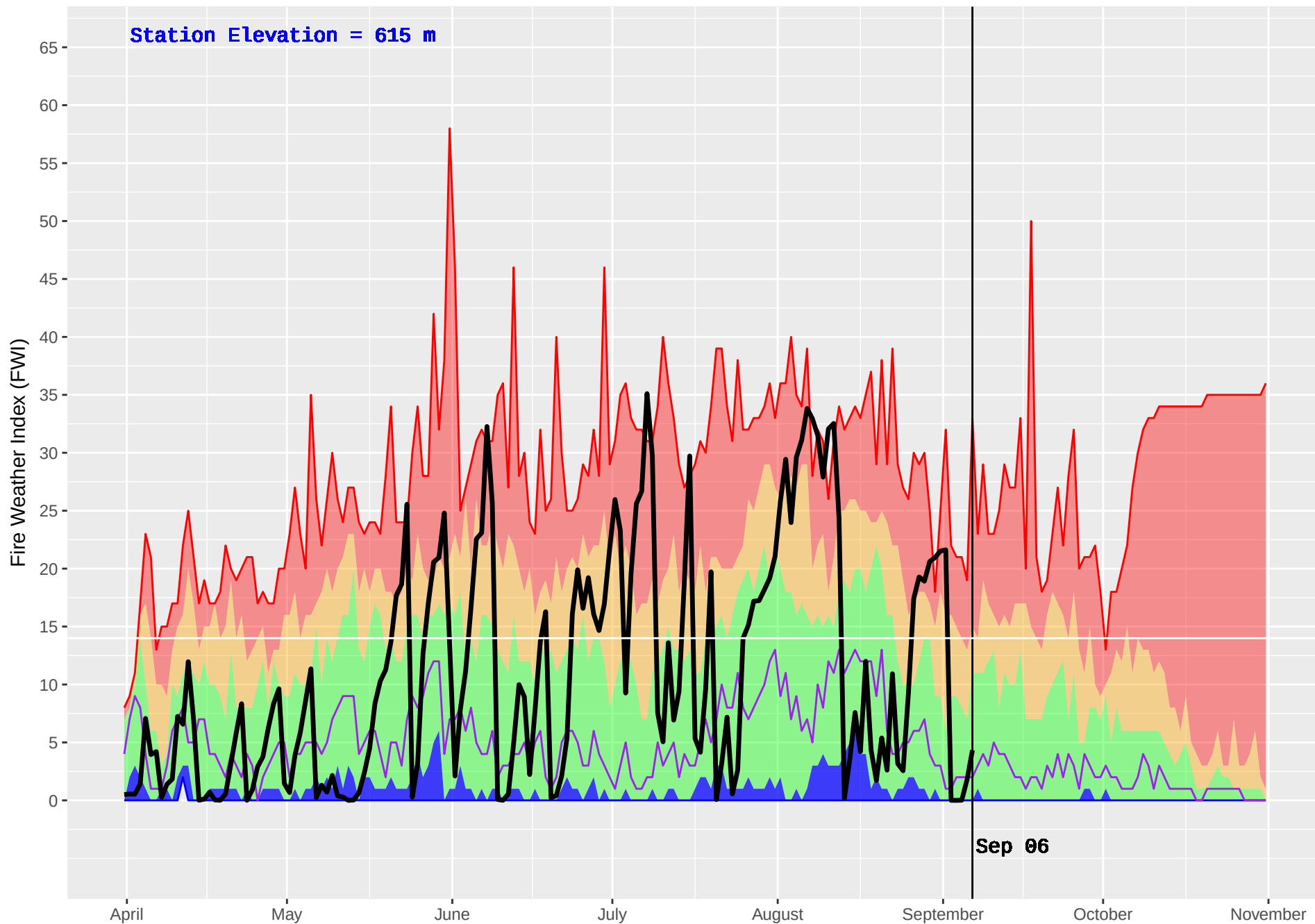
HIXON (187) : Historical (1976–2016) and Current (2017) Noon Fire Weather Index (FWI)
