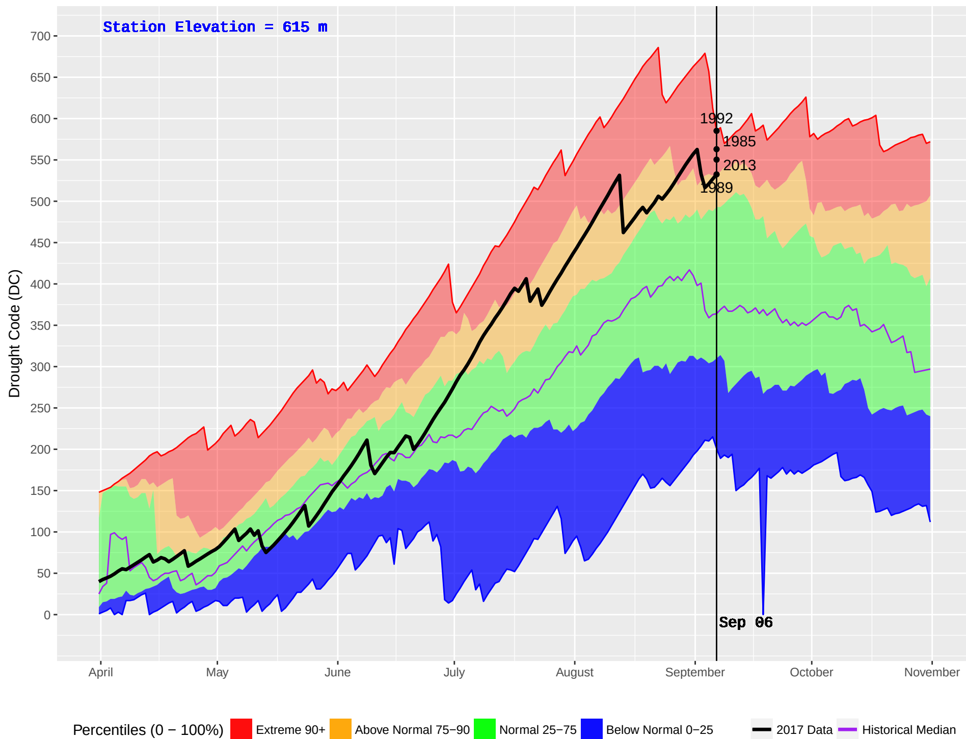
HIXON (187) : Historical (1976–2016) and Current (2017) Noon Drought Code (DC)
