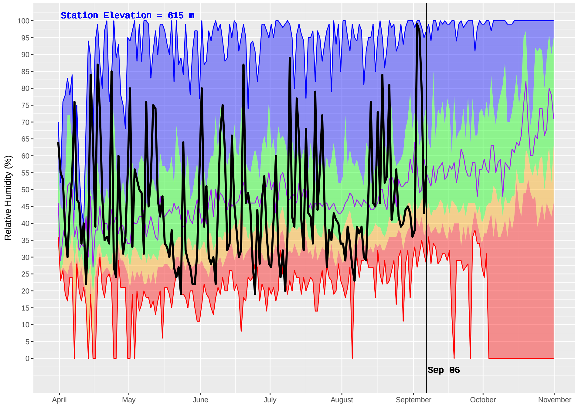
HIXON (187) : Historical (1976–2016) and Current (2017) Noon Relative Humidity
